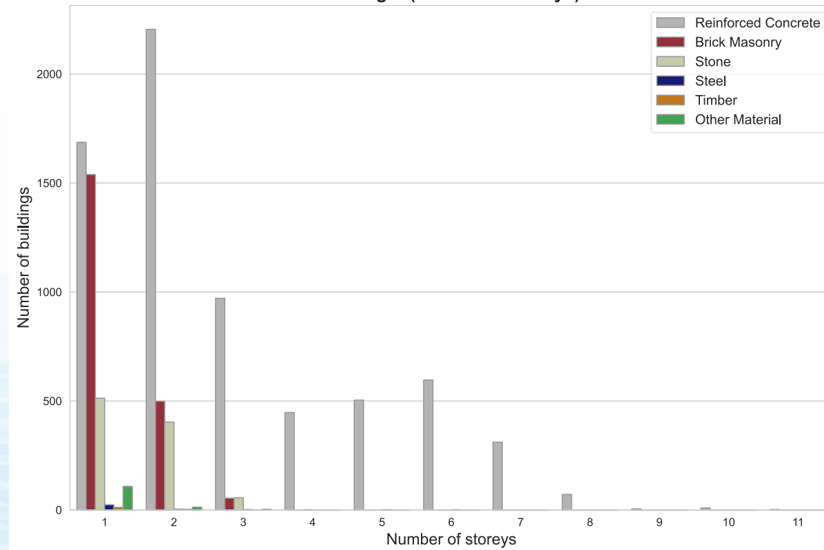
Material vs height (number of storeys) - Xanthi
