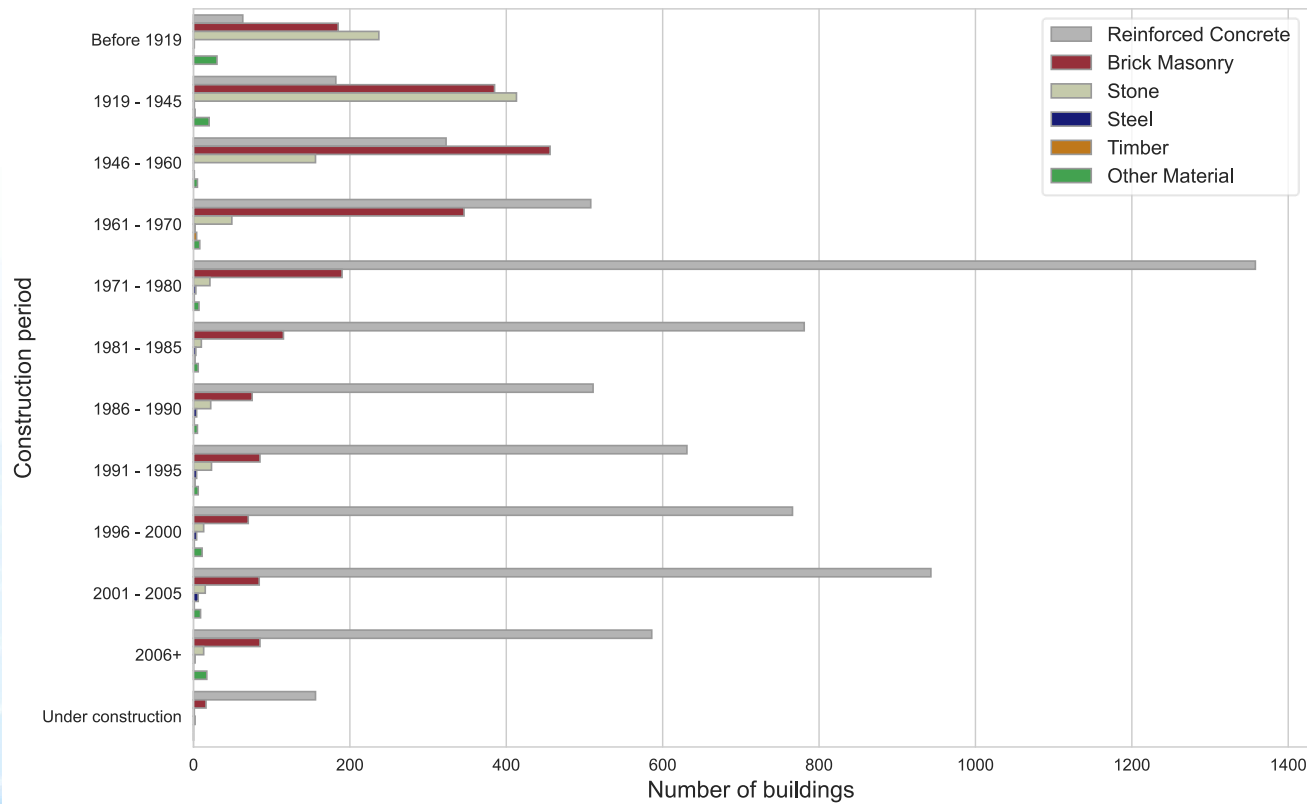
Construction material - Xanthi
