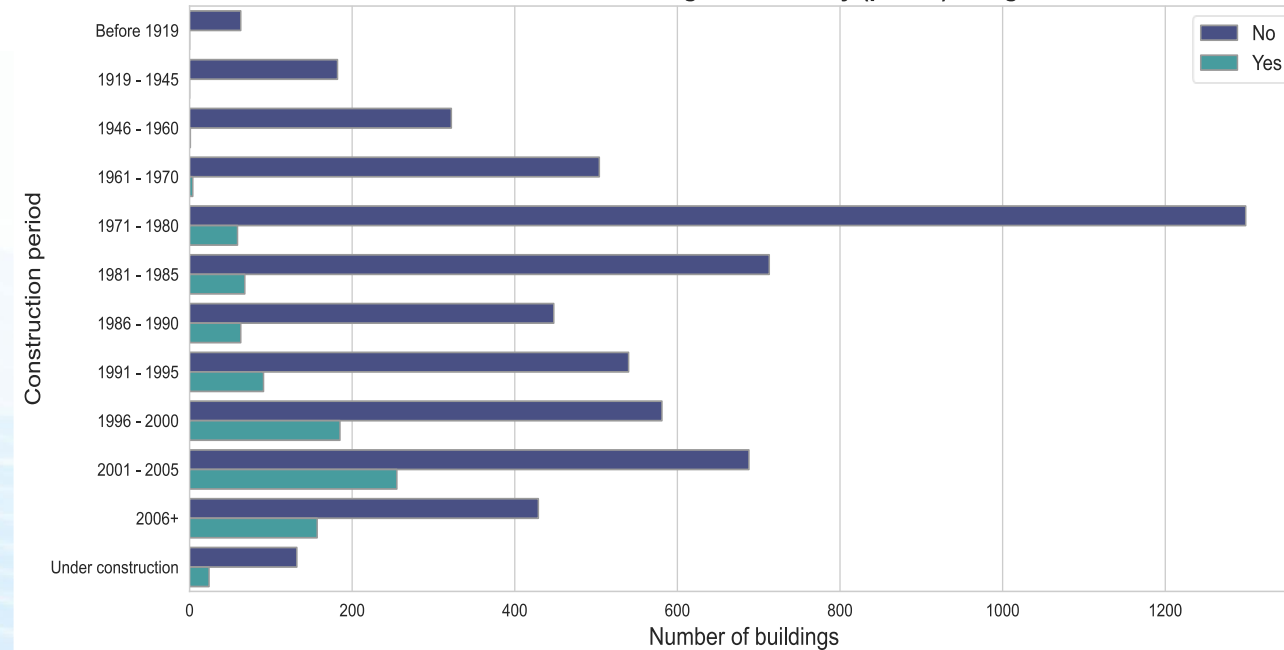
Reinforced concrete buildings: Soft storey (pilotis) vs age - Xanthi
